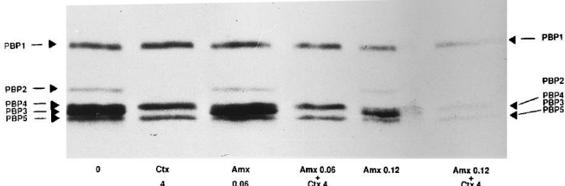
FIG. 5. Saturation of PBPs of JH2-2 with amoxicillin (0.06 and 0.12 µg/ml) alone or in combination. Radioactive benzylpenicillin was used. On this gel, which was run at 4°C, PBP 4 has migrated above PBP 3. Amx, amoxicillin; Ctx, cefotaxime.
