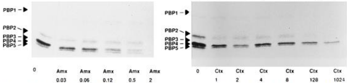
FIG. 4. Saturation of PBPs of JH2-2 by amoxicillin or cefotaxime. Competition experiments with radioactive benzylpenicillin were carried out with increasing concentrations (in micrograms per milliliter) of amoxicillin or cefotaxime. Amx, amoxicillin; Ctx, cefotaxime.
