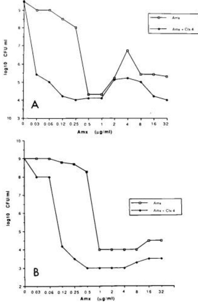
FIG. 1. Synergistic effect between amoxicillin and cefotaxime against JH2-2 on brain heart infusion agar. AMX, amoxicillin; CTX, cefotaxime.
